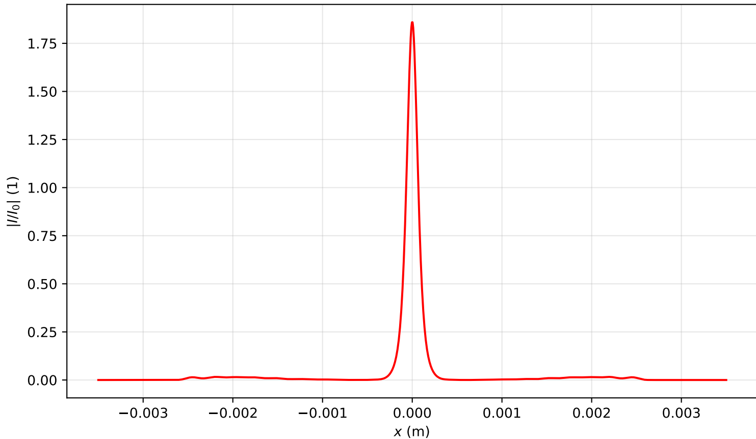
Intensity profile I(x, y = 0, z = 1.751)/I_0 , P_{in}=8.0P_{cr} , artificial time
